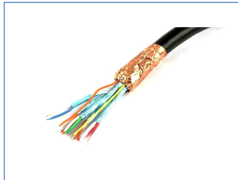
Round HDMI cable
